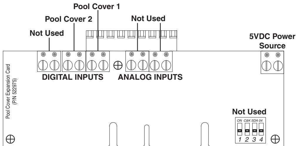
Figure 3. IntelliCenter™ Pool Cover Expansion Card Digital Inputs
