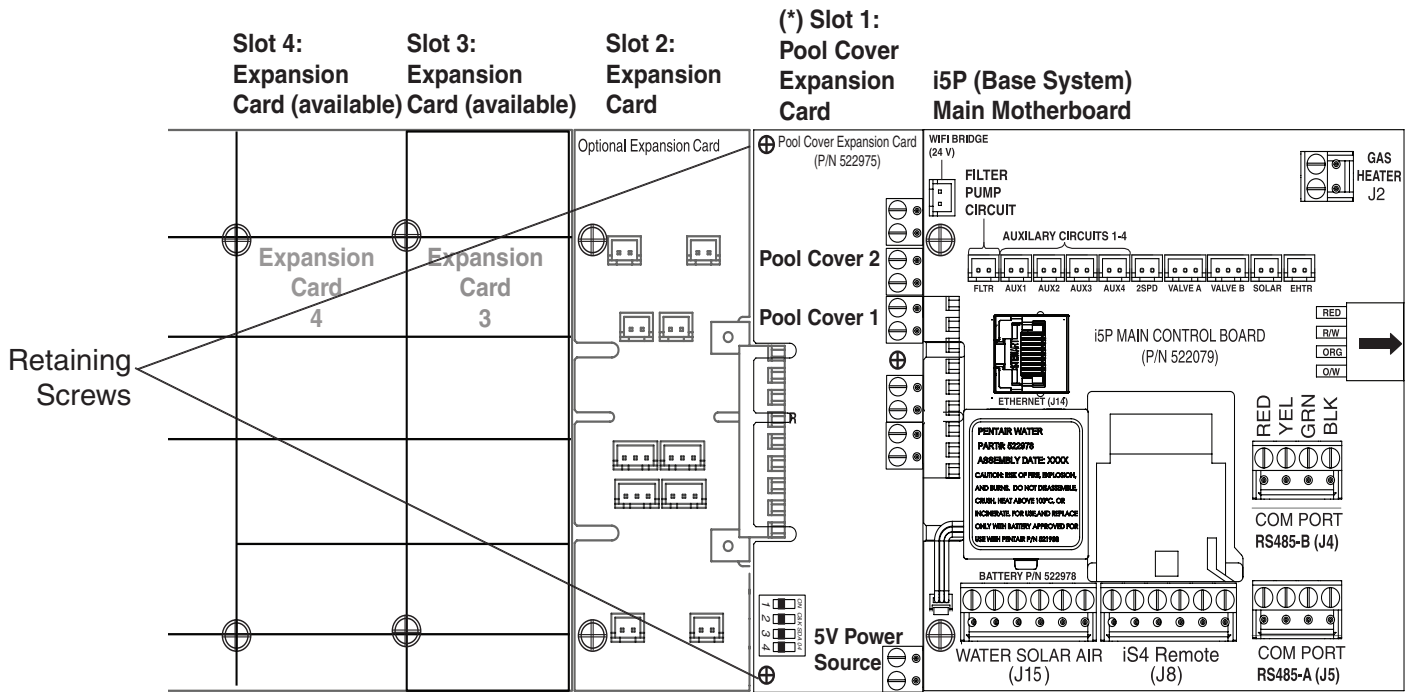
Figure 3. (*) Use SLOT 1 for Pool Cover Expansion Card if no Personality Card is being used, otherwise use SLOT 2, 3, or 4.
