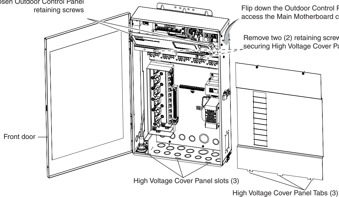
Figure 2: IntelliCenter Load Center Control System Load Center (front view) (High Voltage Cover Panel removed)
