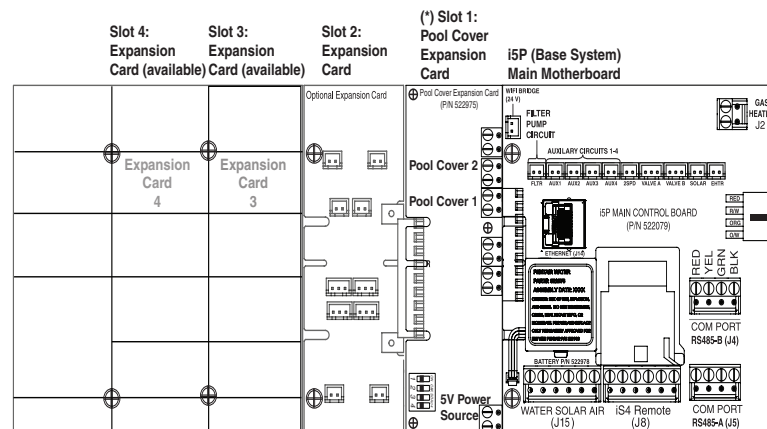
Figure 1: IntelliCenter Control System with Pool Cover Expansion Card Installed (i5P Main Motherboard)
